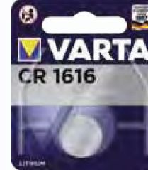
CR1616 3 V - 55 mAh Ø 16.0 - H 1.6 mm bls1 - 10
