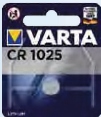
CR1025 3 V - 25 mAh Ø 10.0 - H 2.5 mm bls1 - 10
