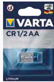
CR1/2AA 3V- 700 mAh 24.9 x 14.45 bls1 1
