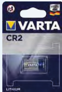
CR2 V 3V- 850 mAh Ø 15.6 - H 27.0 bls1 1
