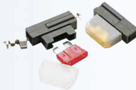
FU.934 - Norm fuse FHA20 2-40A (10)
