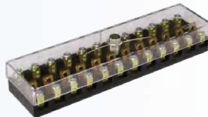
FU.952 - Ceramic Fuse univ. 12P (1)
